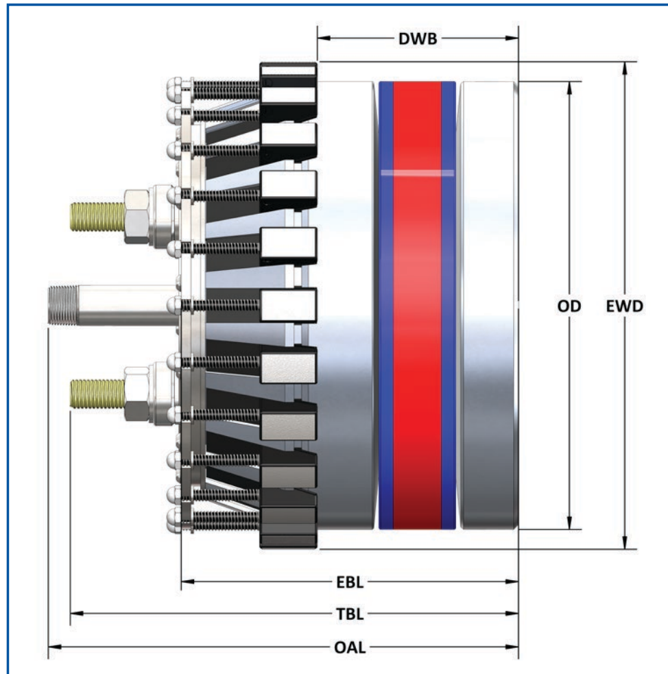
Figure 2: GripSafe ORB Dimensions Diagram
