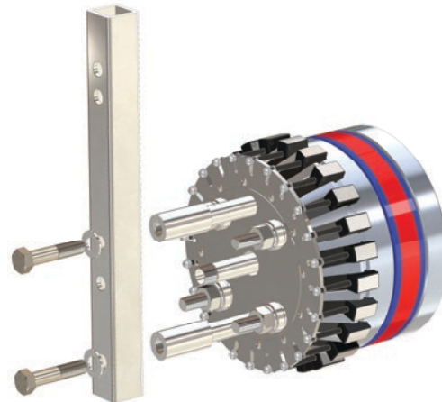
Figure 12: Aligning and Fastening Telescoping Lifting Attachment onto Lifting Standoffs
