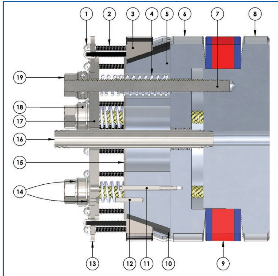
Figure 1: GripSafe ORB Diagram
