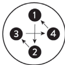
4 Compression Hex Nut Tightening Pattern
