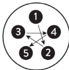
5 Compression Hex Nut Tightening Pattern
