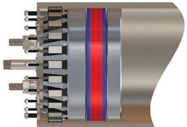
Figure 6: GripSafe ORB Minimum Insertion Depth in a Sectioned Pipe
