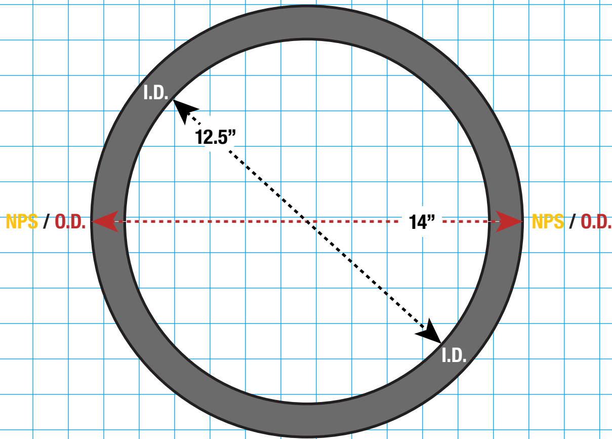
14" SCHEDULE 80 PIPE SIZE & THICKNESS
